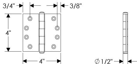
HNG4B Plain Bearing Extruded Hinge 4" x 4" / Each ..... $ 118.00
