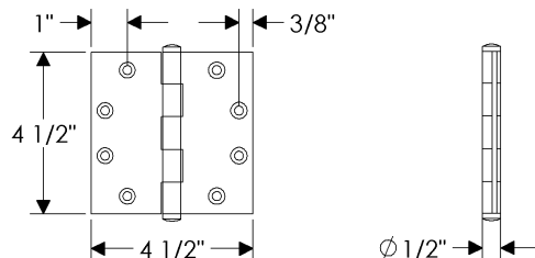
HNG4.5B Plain Bearing Extruded Hinge 4 1/2" x 4 1/2" / Each ..... $ 130.00
