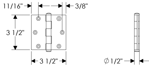
HNG3.5B Plain Bearing Extruded Hinge 3 1/2" x 3 1/2" / Each ..... $ 108.00
