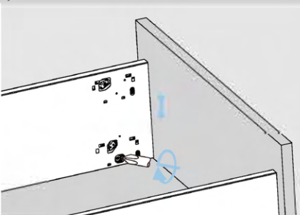
Up&down adjustment
