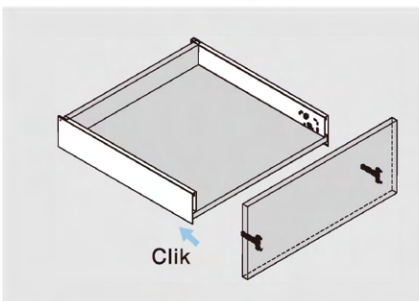
Front assembly
