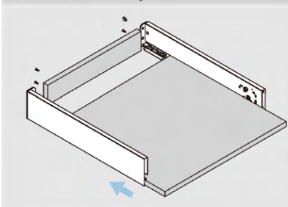
Back and Bottom assembly
