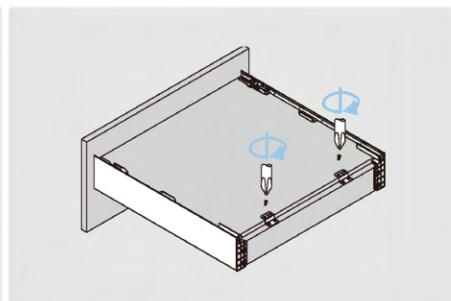
Fixing-brackets assembly
