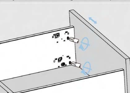
Left&right adjustment
