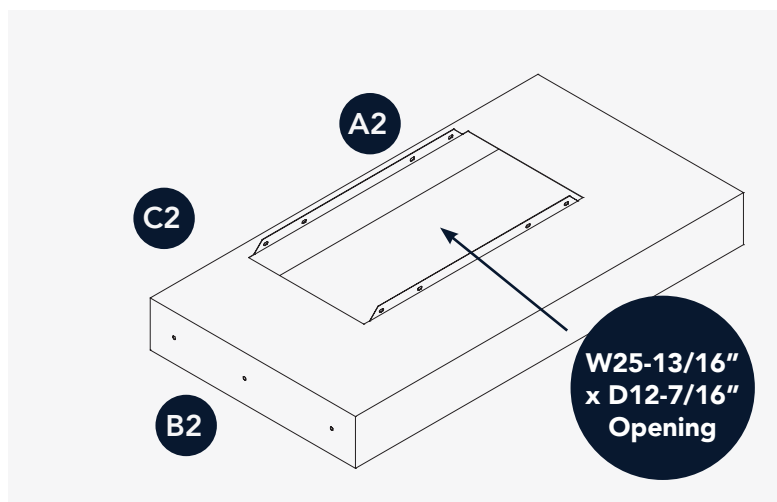
Liners Specifically Designed for Sirius 960CFM Ventilator
