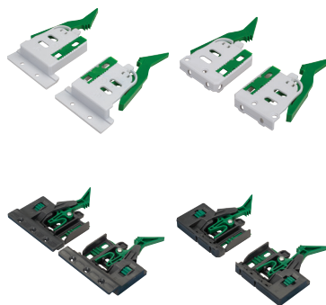
1D and 2D Front Locking Devices
