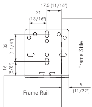
Rear Bracket for Face Frame
