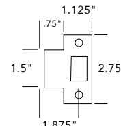
Standard Box T-Strike
