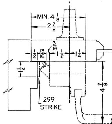
88 Series Single Door w/ 299 Strike
