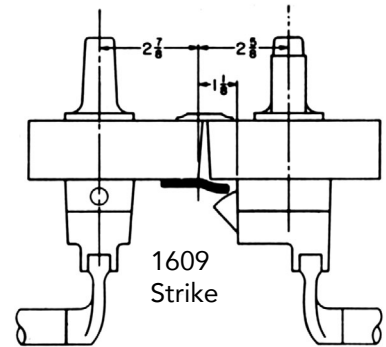
88 Series Double Door w/ 1609 Strike
