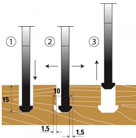
Vertical Mechanical Drive: Cuts vertical movement into plunge cut allowing installation of Clamex connectors
