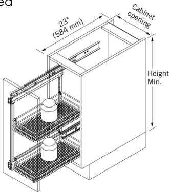
Cabinet dimensions allow 23" Depth
