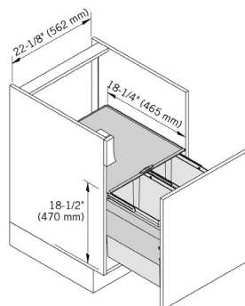
Cabinet Dimensions
