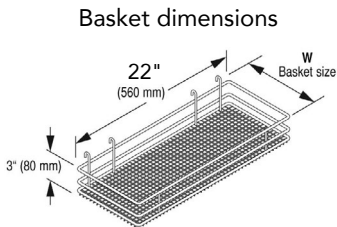
Two Basket widths available
