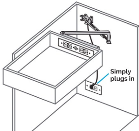
Electrical Connection
