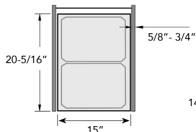
Product Dims
