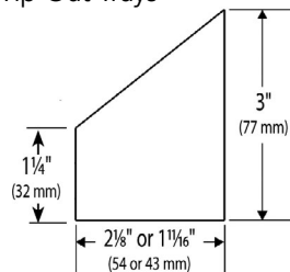
Regular and Slim Series Stainless Steel Tip-Out Trays
