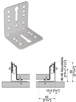
Bottom Mount
