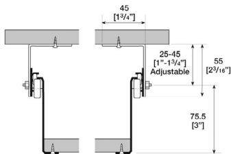
Top Mount
