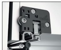
Rear Tilt Bracket
