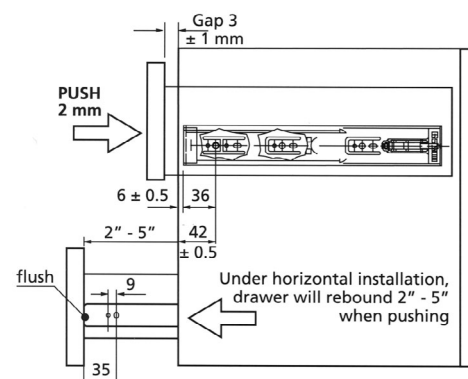
Side Mount "Push" Slide
