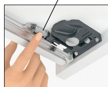
Front Clip: - Side adj. - Height adj.
