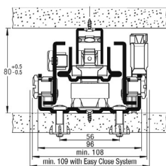
bottom slide
