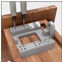
F70-JIG for Clips/ Rear Hole
