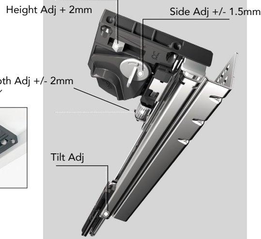
Front Clip: - Side adj. - Height adj.
