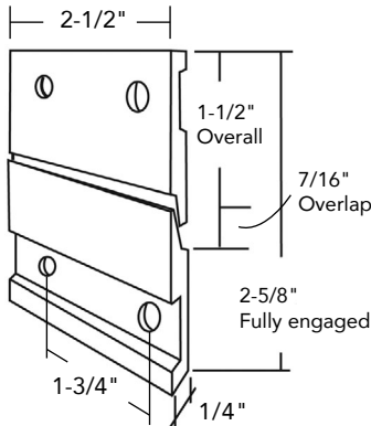
HC2 Clips - 2-1/2" width Sold per pair
