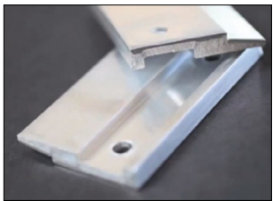
HC2 Clips - 2-1/2" width Sold per pair
