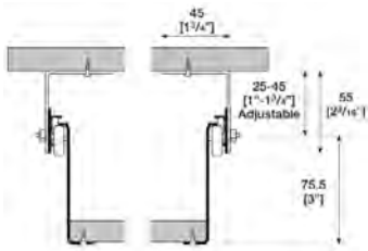
Top Mount
