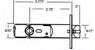
2-3/4" Backset
