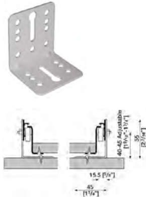
Bottom Mount
