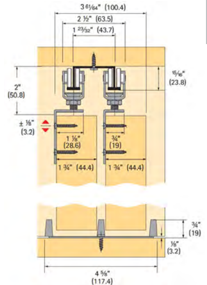
For Doors 1-3/4"
