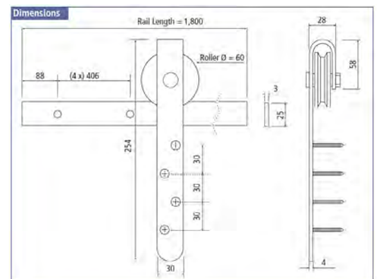
FT-MINI - Flat Rail Surface Mount Specs
