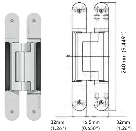
TE-640-3D / 440 lbs/pr. For high performance commercial doors
