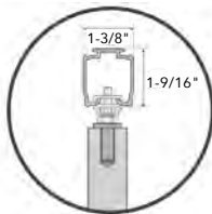
Track Installation
