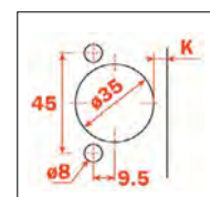
Knock-In Dowel, Rapido, Logica
