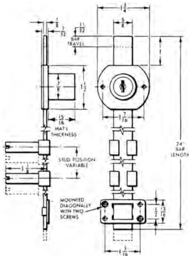
Mounting Hole: Additional 7/8"x1/8" deep dado for bar required on inside of panel
