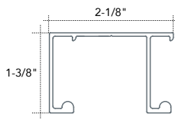
Track U28-35 For Door Thickness: 3/4" - 1-3/8"
