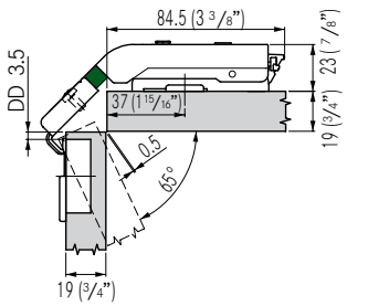
19mm door thickness with base plate height 0
