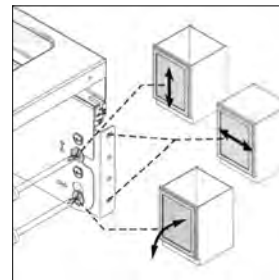
Door bracket adjustment: Tilt, Height, Overlay
