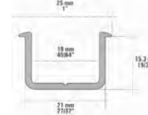
Track U21
