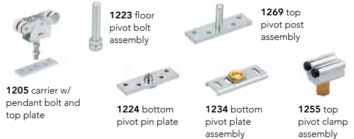
(2) 1205 four-wheel carrier w/ pendant bolt and top plate
