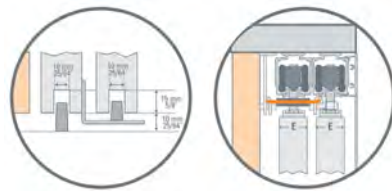
Guide Installation 13/16" > E < 1"
