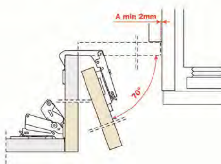
C2AYA99 hinge movement and maximum opening width
