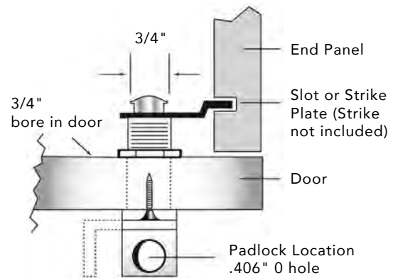
Closed position
