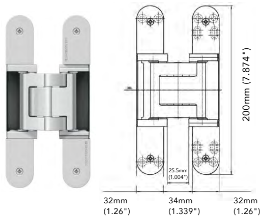
TE-540-3D A8 / 200 lbs/pr. For doors with claddings of up to 8mm (.315")
