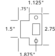
Standard Box T-Strike
