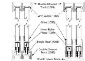
Recessed Mount
