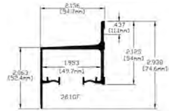
Single Track w/Fascia
