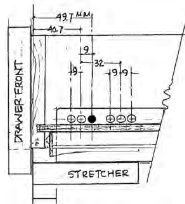
19mm (3/4") Setback (6mm + material thickness)
