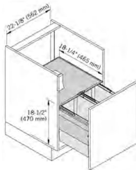
Cabinet Dimensions
