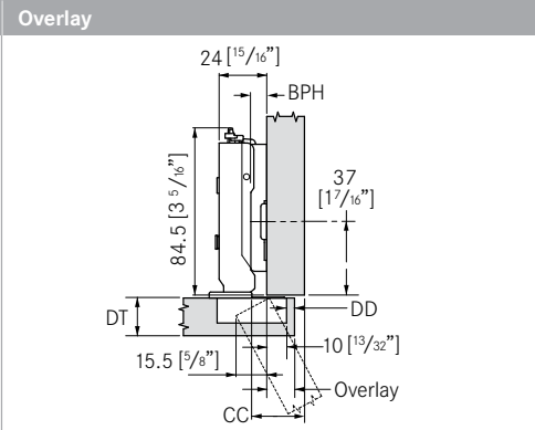
Drawing shows Tiomos with a base plate height (BPH) 02.
