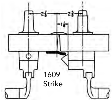
88 Series Double Door w/ 1609 Strike
