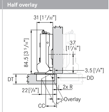
Drawing shows Tiomos with a base plate height (BPH) 02.
