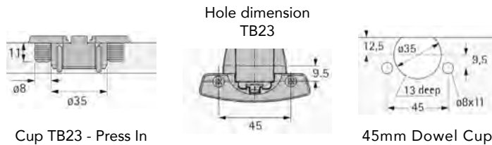
Cup TB23 - Press In
