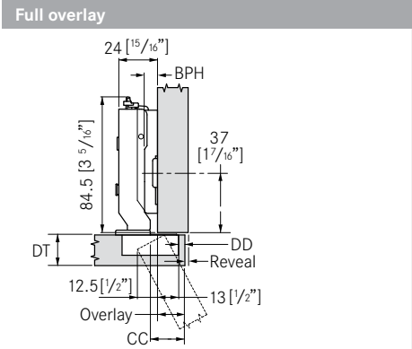
Drawing shows Tiomos with a base plate height (BPH) 02.
