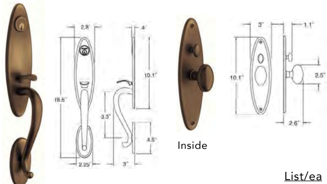
Entry Trim
