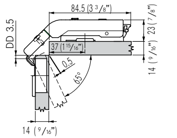
14mm door thickness with base plate height 0
