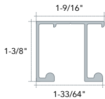
Track U28 For Door Thickness: 3/4" - 7/8"
