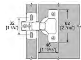
Overall Dimensions
