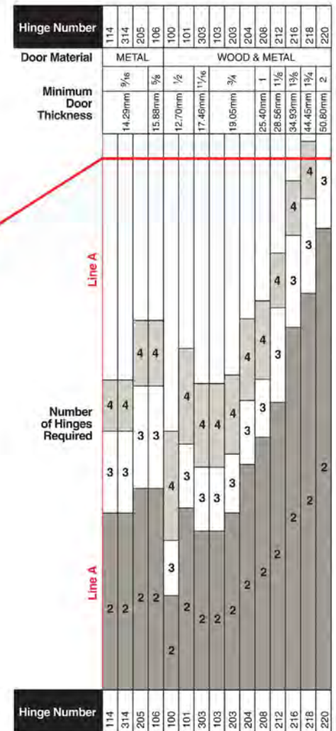
Selector chart based on theoretical values. For extreme conditions consult factory.
