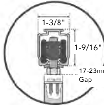
Track Installation
