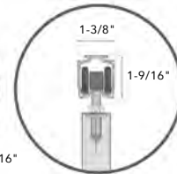
Track Installation
