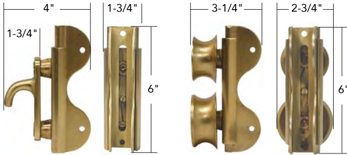
No. 230 Hook Slide
