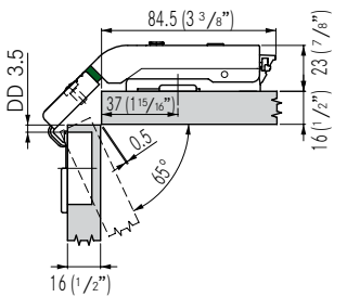
16mm door thickness with base plate height 0
