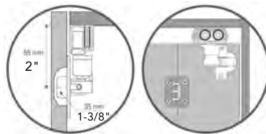
Carrier Installation
