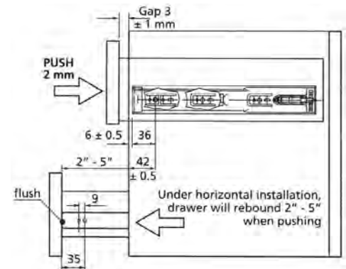
Side Mount "Push" Slide
