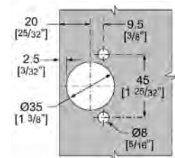
Drilling Pattern
