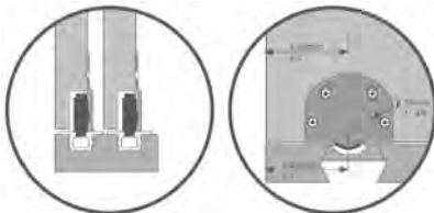
Carrier Installation 35mm edge bore
