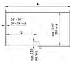
Cabinet Dimensions
