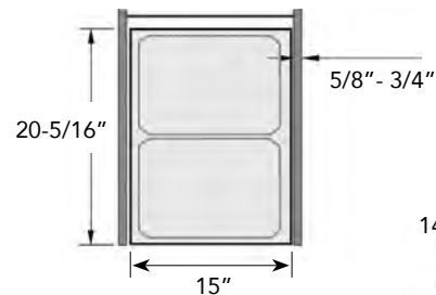
Product Dims
