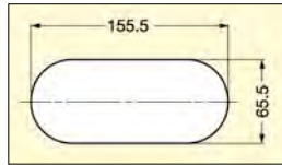
Hole Size
