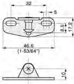
Arm Mounting Plate
