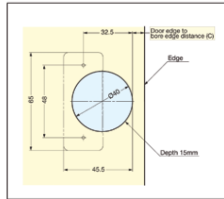
Bore Dimensions
